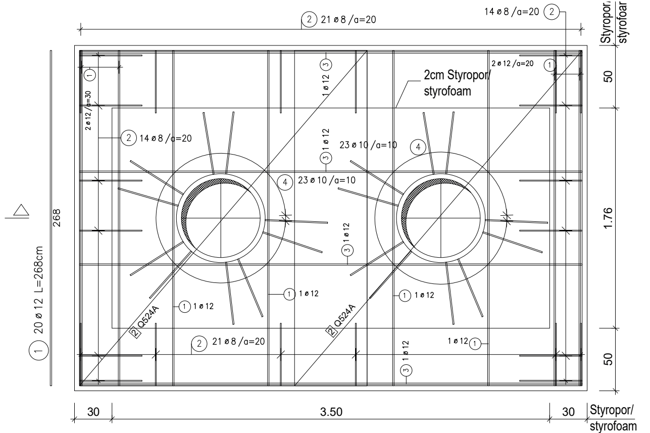
Bottom view
