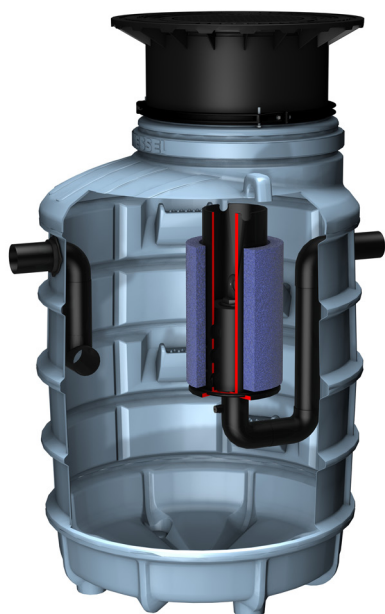
3.5 Illustration: KESSEL-koalescensavskiljare EasyOil Schakt FB 1000, NS 3
